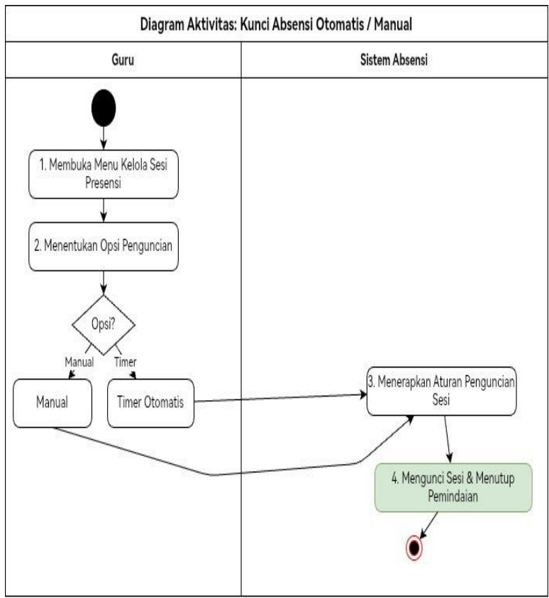
Activity Diagram: Kunci Absensi Otomatis / Manual
