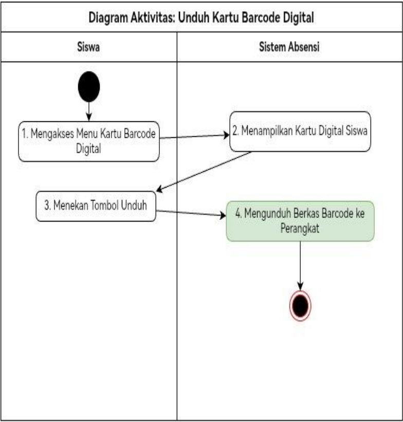
Activity Diagram: Unduh Kartu Barcode Digital
